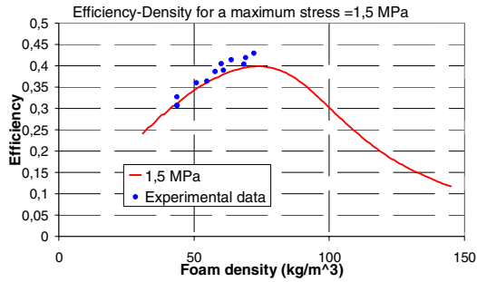
Figure 31. Experimental efficiency points at a defined stress of 1.5 MPa and model curve for EPS foams.
