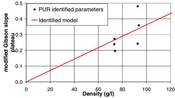
Figure 25. Linear density dependence law of the slope h parameter identified for the PUR foams.
