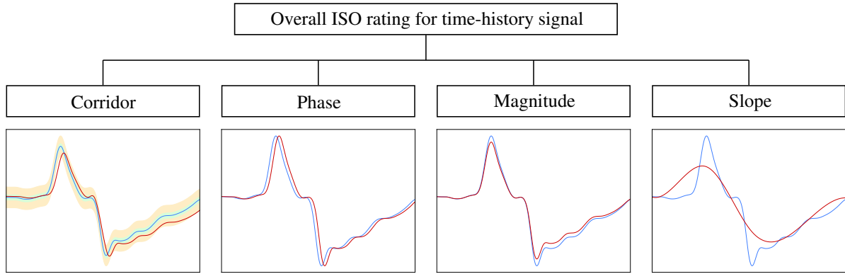
Figure 2. Composition of the overall score from the scores of different sub-metrics by means of the ISO/TS 18571 [1]. The diagrams show an example for each sub-metric with the reference (blue) and the comparison signal (red).
