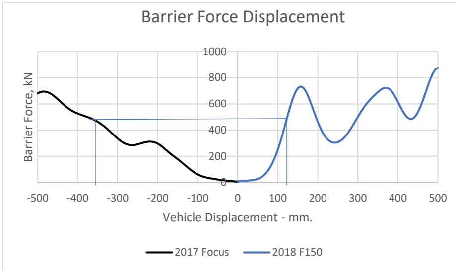
Figure 12. Stiffness comparison of the Focus vs F 150
