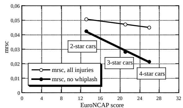
Figure 3. Risk of fatality or permanent disability, mrsc, versus Euro NCAP scores.
